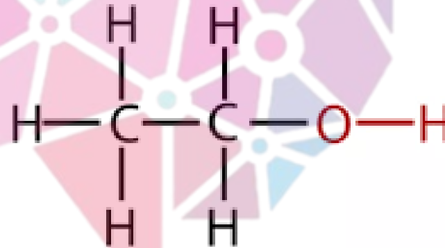
Structural formula
